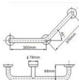
15.211.ST 300x300mm
